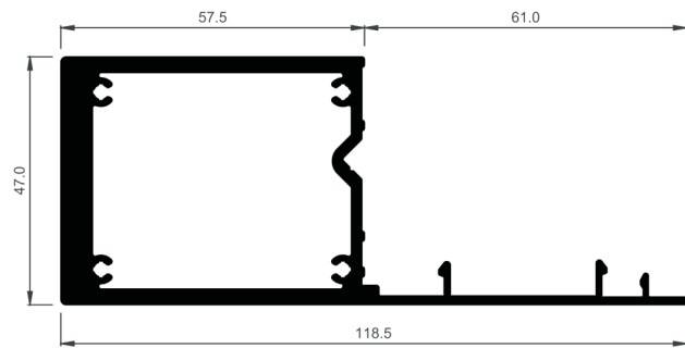
COR-4751 47x57,5 mm reinforcement
