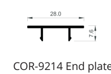
COR-9214 End plate
