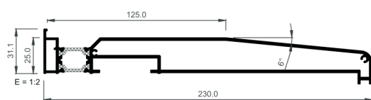
COR-3838 Subcill 230 mm
