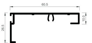
COR-4743 Fixed sash frame cover
