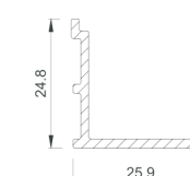
COR-4702 One rail frame with fixed isolation
