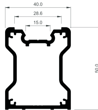
COR-4750 Reinforcement 40x50 mm
