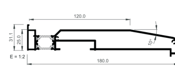
COR-3837 Subcill 180 mm
